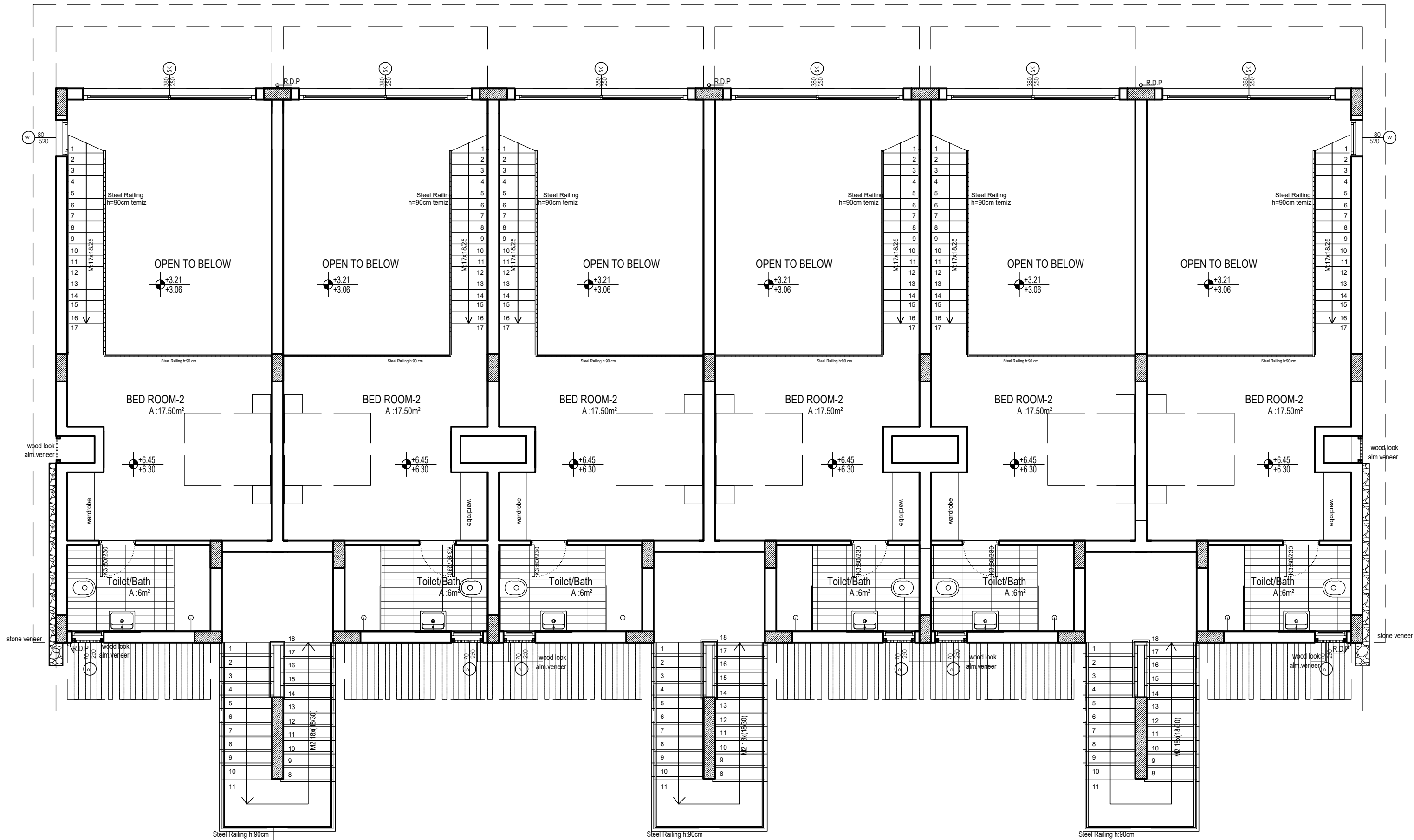
B BLOCK MEZANINNE FLOOR
