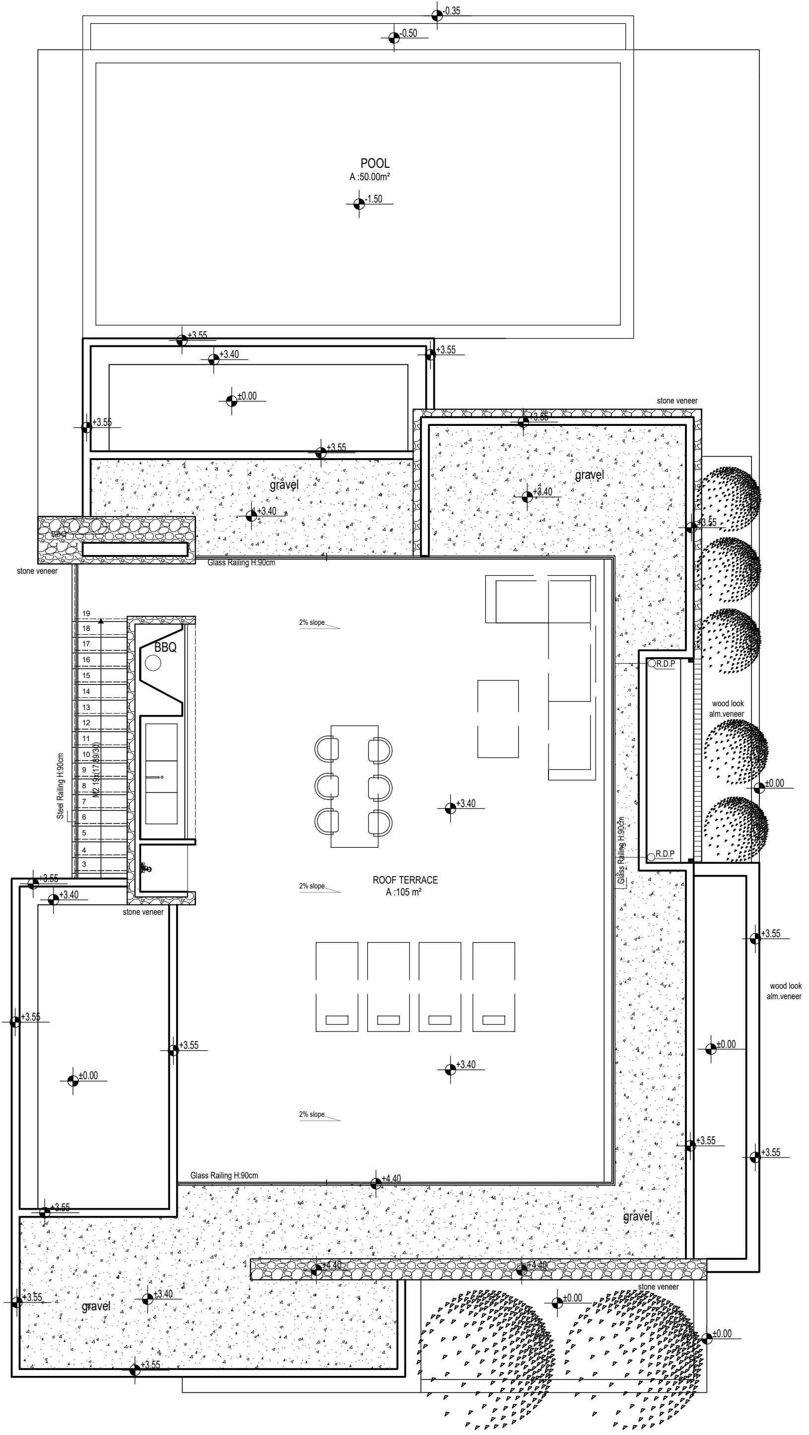
BUNGALOW ROOF PLAN
