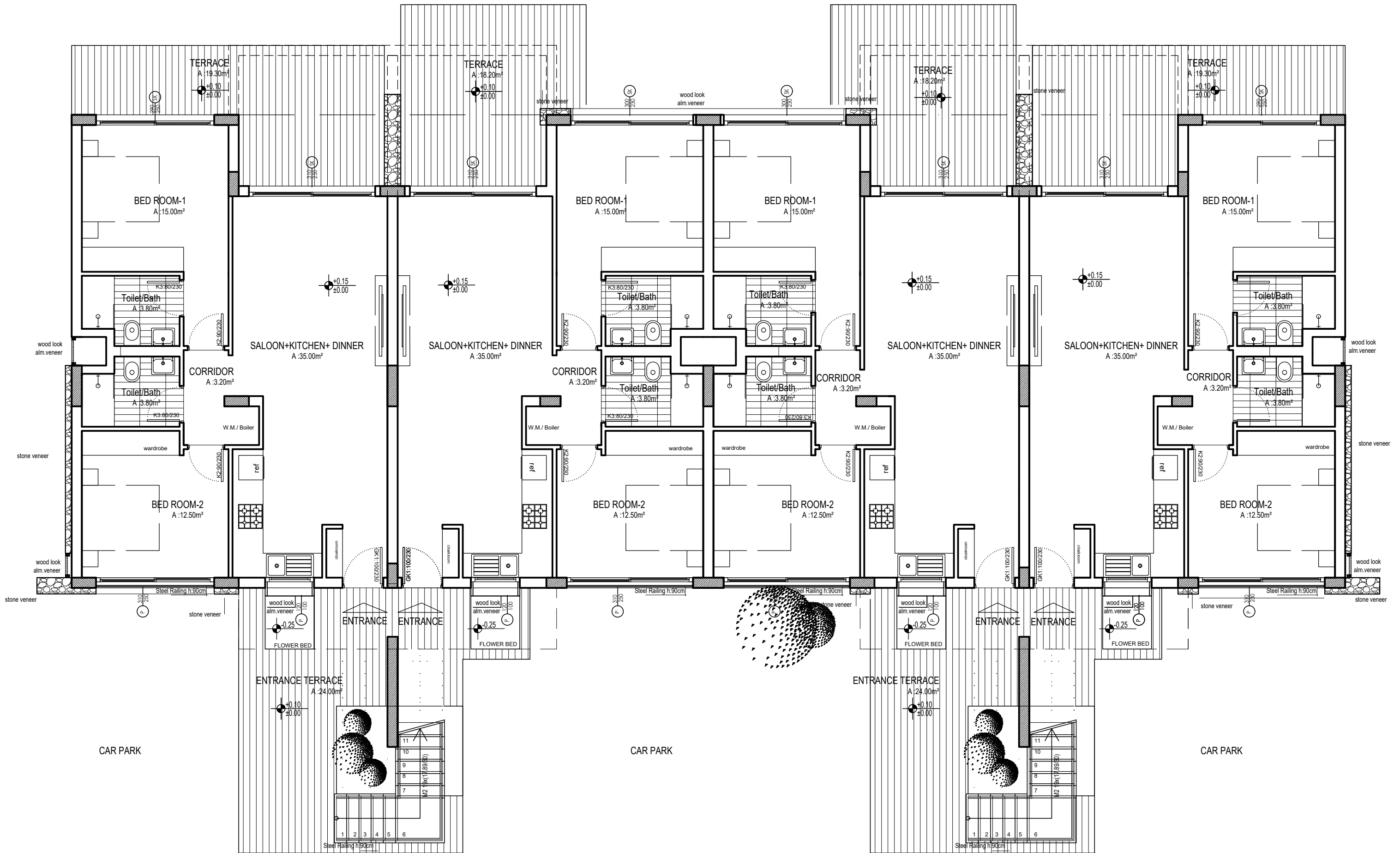
A BLOCK 2+1 GROUND FLOOR
